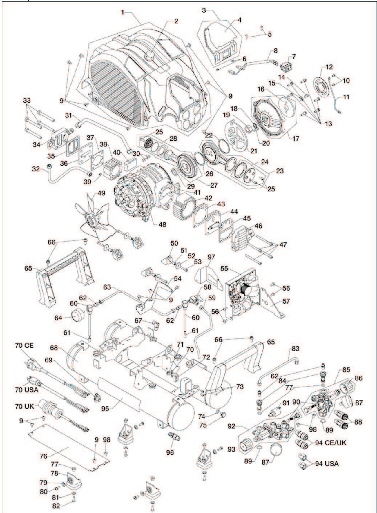
8-1. Exploded View for AKHL1260E
