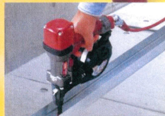
Metal Track to Concrete Ceiling (Ideal Super Light & Compact Tool for Overhead Use)
